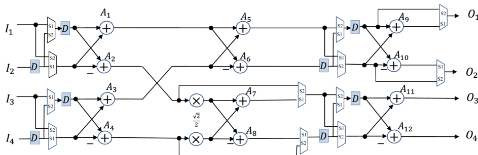
Figure 12. Folded 8-point 4-parallel RFFT.
