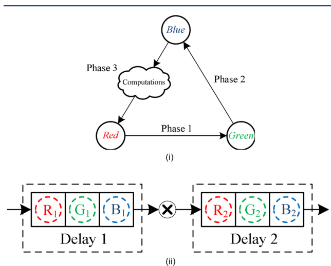
Figure 9. (i) Implementing delay elements using the 3-phase asynchronous scheme. (ii) Cascaded delay elements implemented using the asynchronous scheme.
