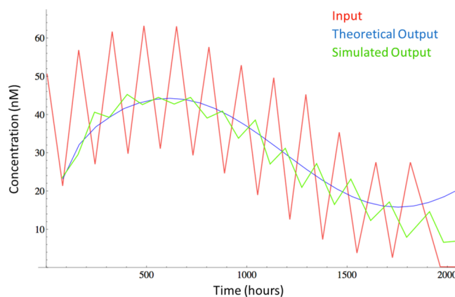
Figure 16. Simulation results for the DNA implementation of the asynchronous moving average filter.
