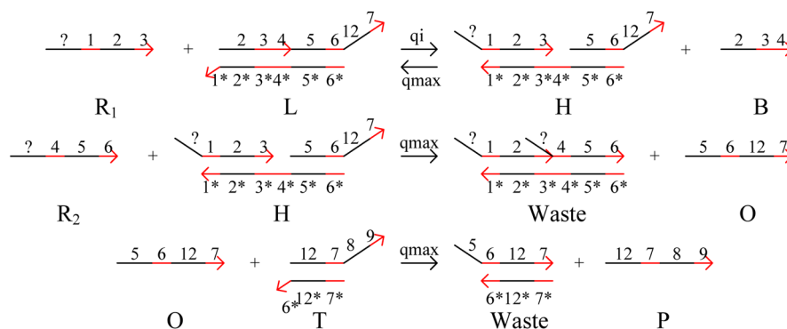
Figure 14. Example of DNA strand displacement.
