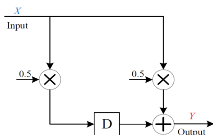
Figure 1. Circuit diagram for the moving-average filter.
