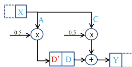
Figure 3. Synchronous implementation of the moving-average filter.
