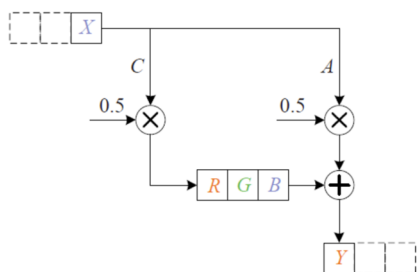
Figure 5. Asynchronous implementation of the moving-average filter.
